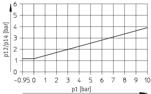
MFH-3-1/2-S
