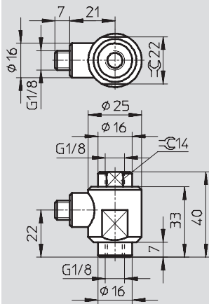
Pneumatic connection G 1 / 8
