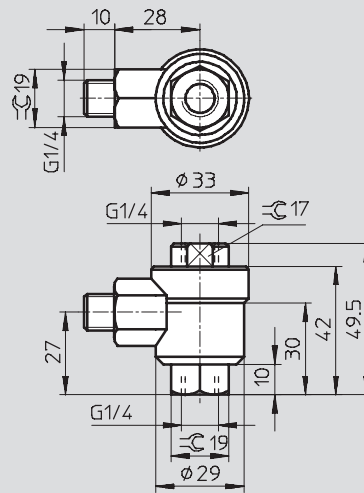
Pneumatic connection G 1 / 4
