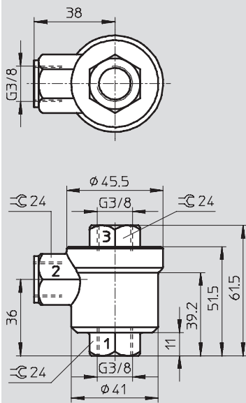
Pneumatic connection G 3 / 8
