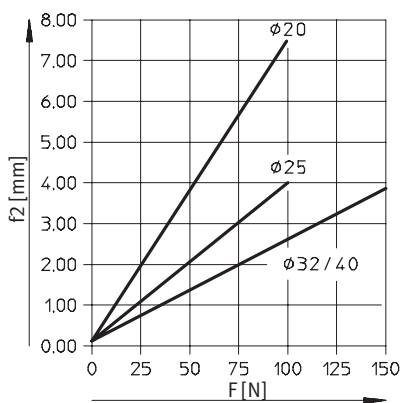
Hub 400 mm
