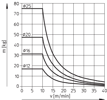
DFM-12 ... 25-GF Hub < 30 mm
