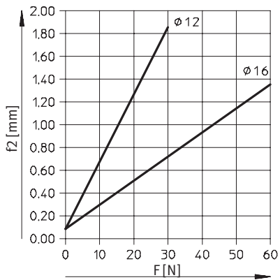
Hub 200 mm
