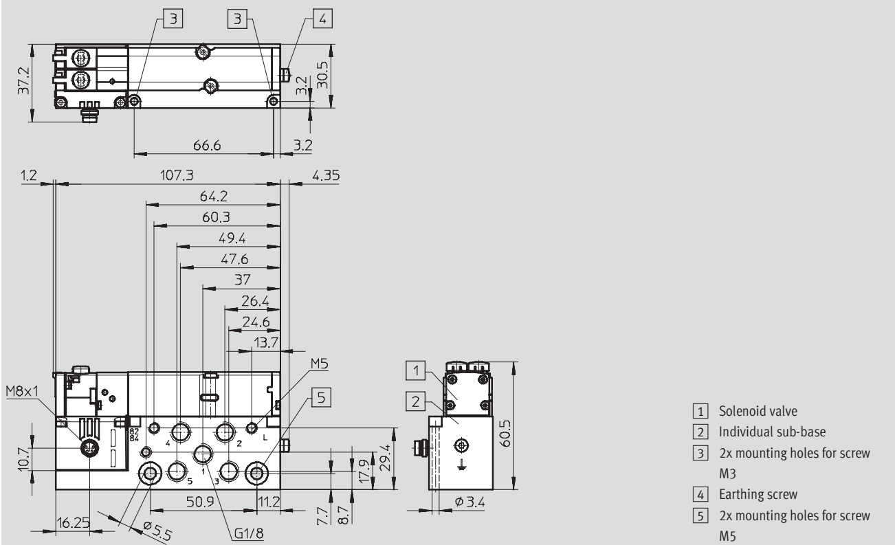
MPA2 valve on individual sub-base
