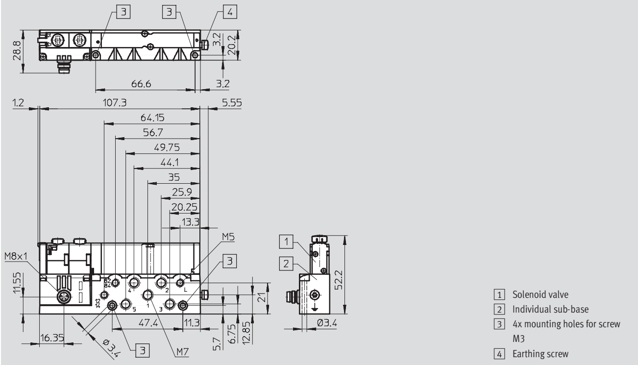
MPA1 valve on individual sub-base
