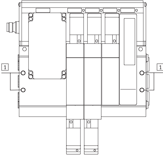
1 Mounting through holes for M6 hexagonal-head bolts
