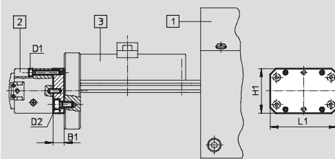
Adapter kit HAPG38/-54/-55/-57
