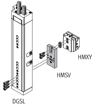
Direct mounting
