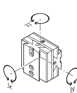
Mass moments of inertia Fig. 2
