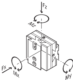
Max. permissible static characteristic load values Fig. 1
