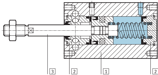
Sectional view EMM(L) – Pushing Sectional view EMM(L)Z – Pulling
