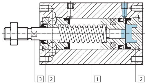
Sectional view EMM(L) – Pushing Sectional view EMM(L)Z – Pulling
