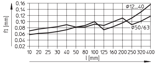
DFM-GF with 2 bearings per guide rod
