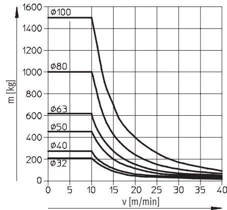
DFM-32 ... 100-GF Stroke < 50 mm
