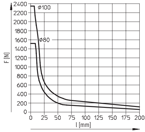
DFM-80 ... 100-KF Stroke 25 mm
