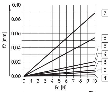
Piston \varnothing 16 mm
