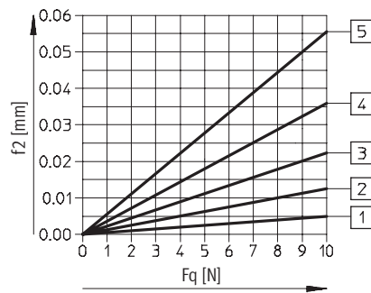
Piston \varnothing 10 mm
