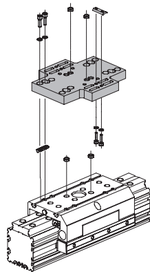
Direct mounting
