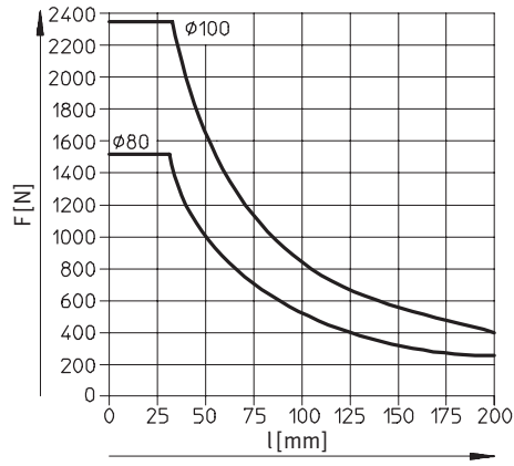
DFM-80 ... 100-GF Hub 25 mm
