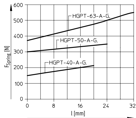
Piston \varnothing 40 ... 63
