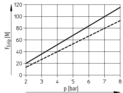
HGDS-20 (max. lever arm x 70 mm)
