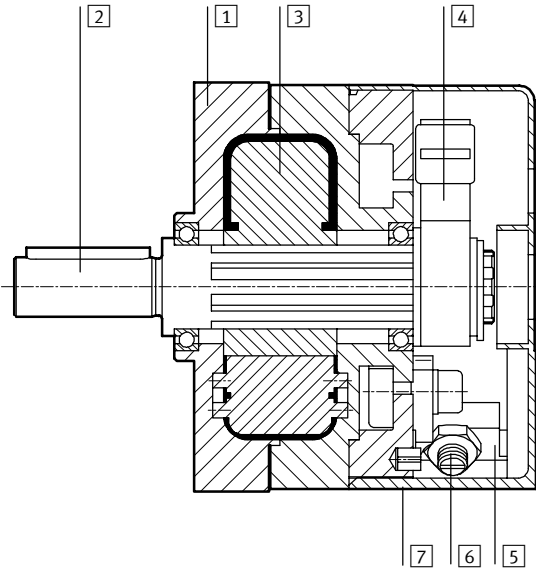
Sectional view of swivel module DSM
